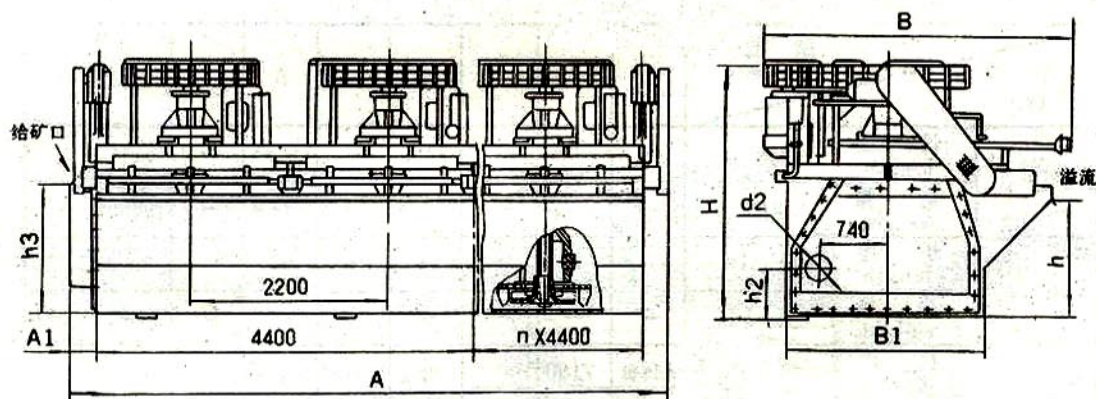
XJ-58 浮选机外形图 diagram of floatation machine
