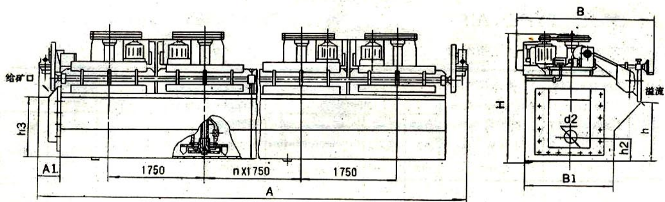
XJ-11 浮选机外形图 XJ-28 diagram of floatation machine
