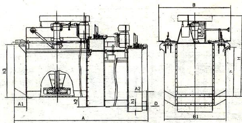
XJC-160 充气搅拌式浮选机 diagram of air-agitation floatation machine
