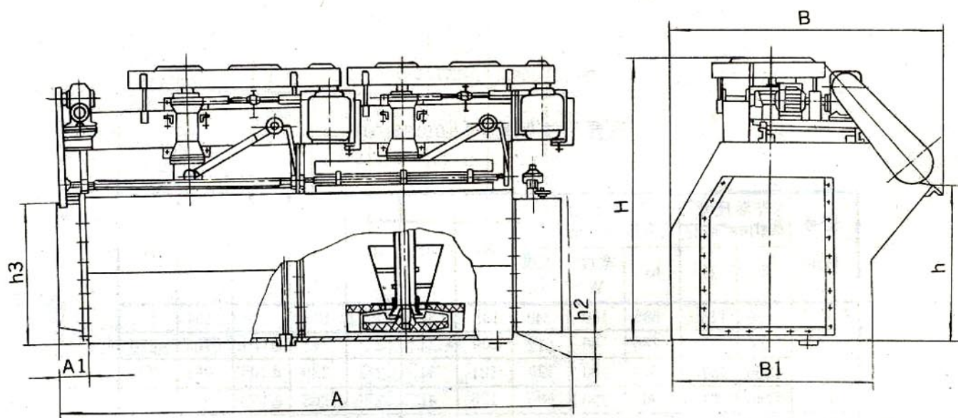
充气搅拌浮选机外形图 XJC-40 diagram of air-agitation XJC-80 floatation machine
